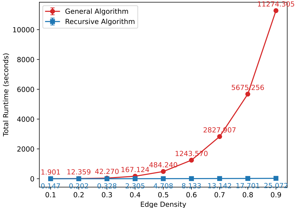
Total Runtime with Basis Tracking (200 realizations per density)
